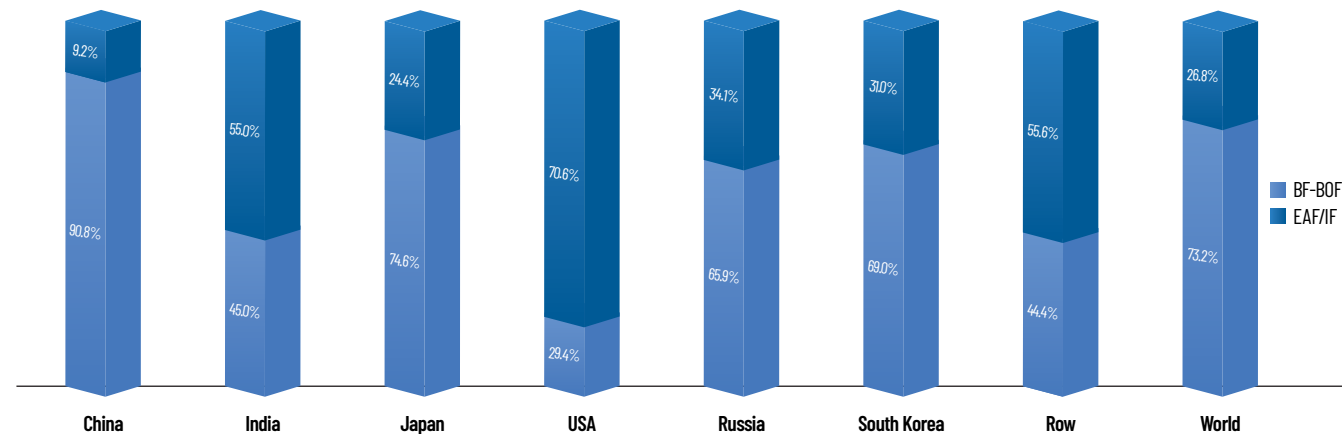
Route wise Production share (Global) 2021
