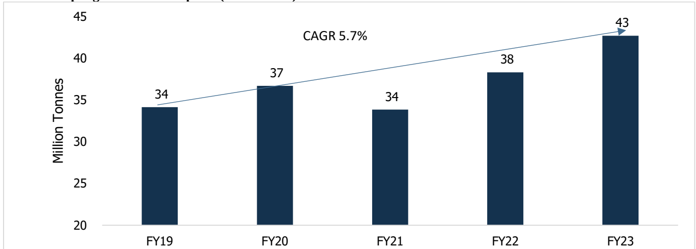
Chart 27: Sponge Iron Consumption (FY19-FY23)
