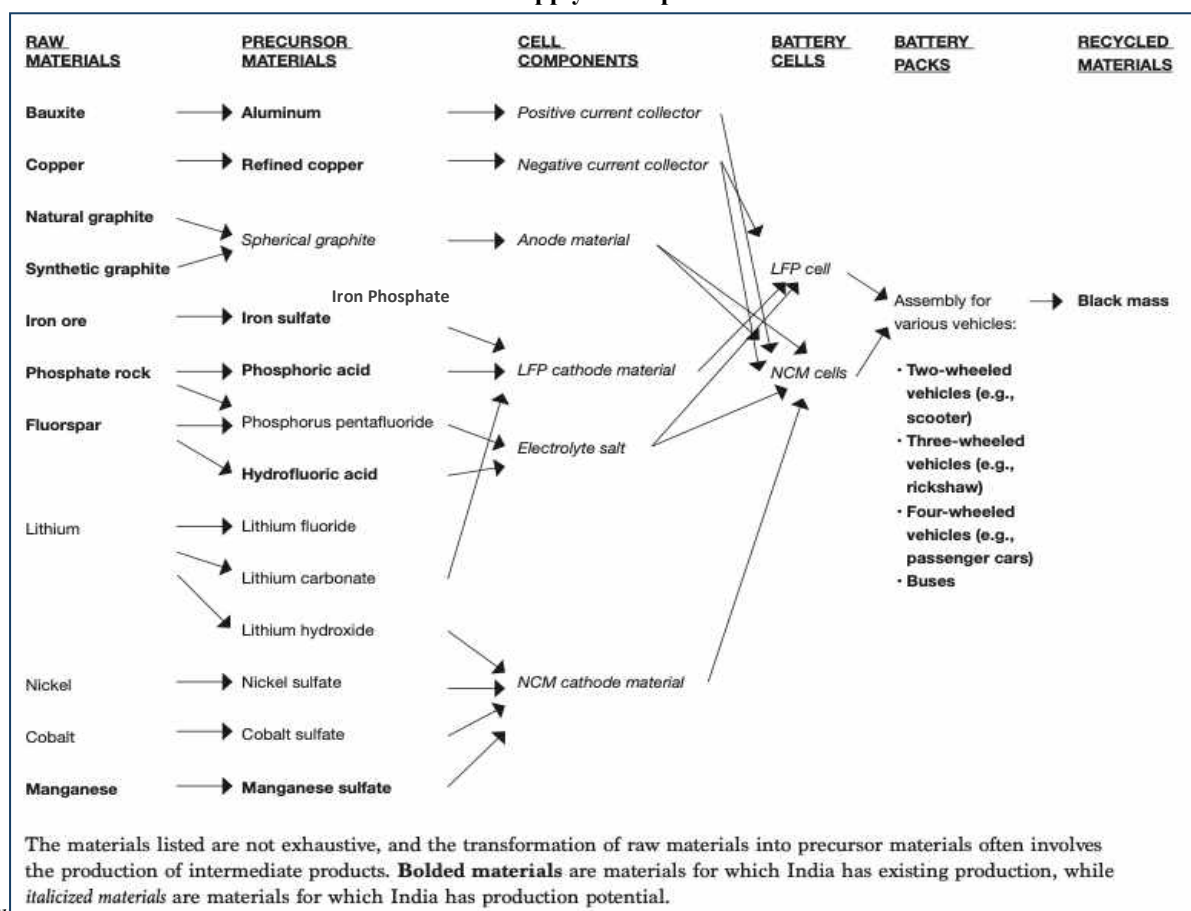
LFP and NMC supply chain process flow India focus
