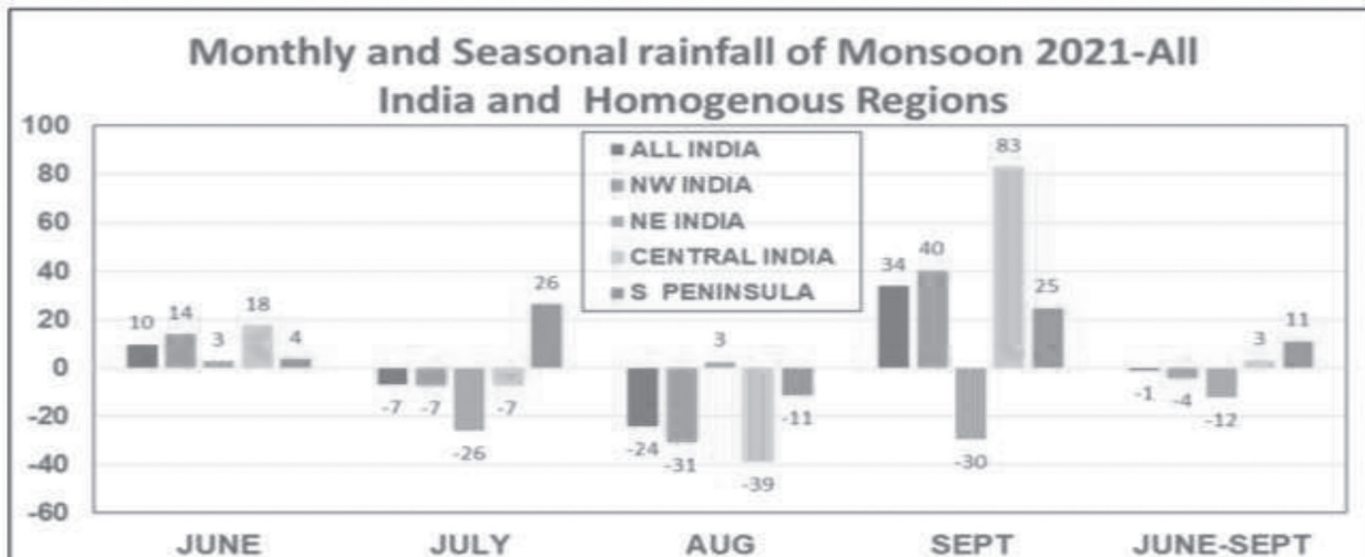
Fig.2. Monthly and seasonal monsoon rainfall of 2021 over Broad homogenous region and Country as a whole in% departure.
