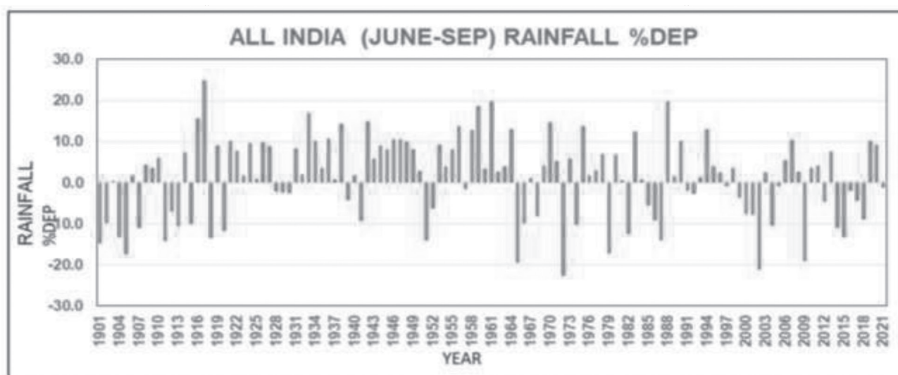
Fig. 1. All India seasonal Monsoon rainfall in% departure from normal
