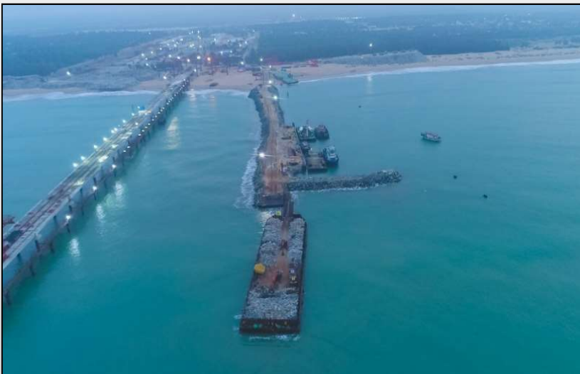
Haldia Inland Waterways – Loadout Jetty with Barge
