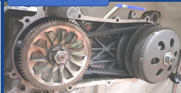
CVT ASSY.
