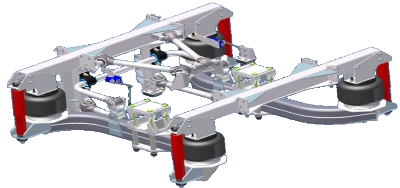
3) Air Suspension
