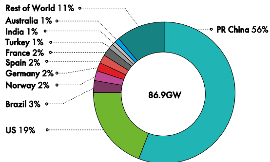
New installations onshore (%)
