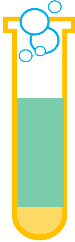
Formic Acid
