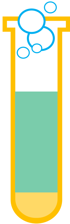
Acetic Acid
