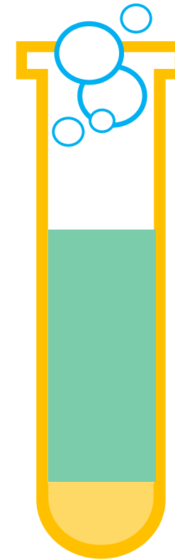
Di-Calcium Phosphate
