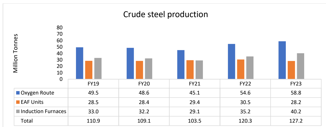
Chart 36: Technology-Wise Crude Steel Production (FY19-FY23)
