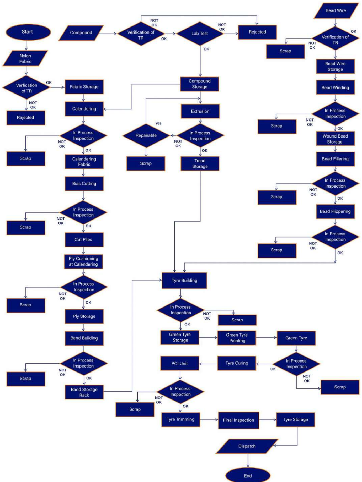
Tyre Process Flow Diagram
