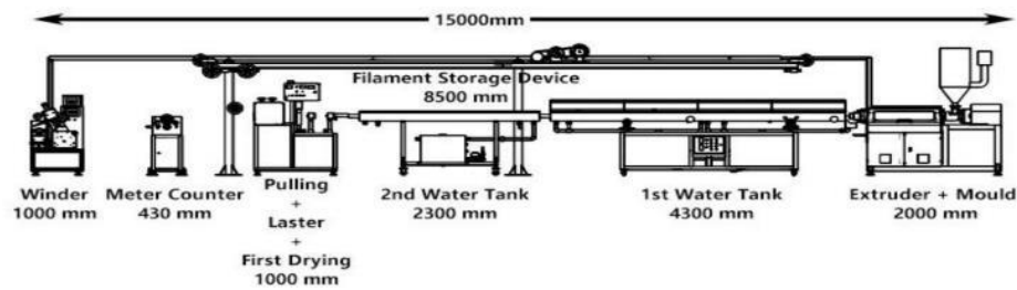
Machine Drawing :
