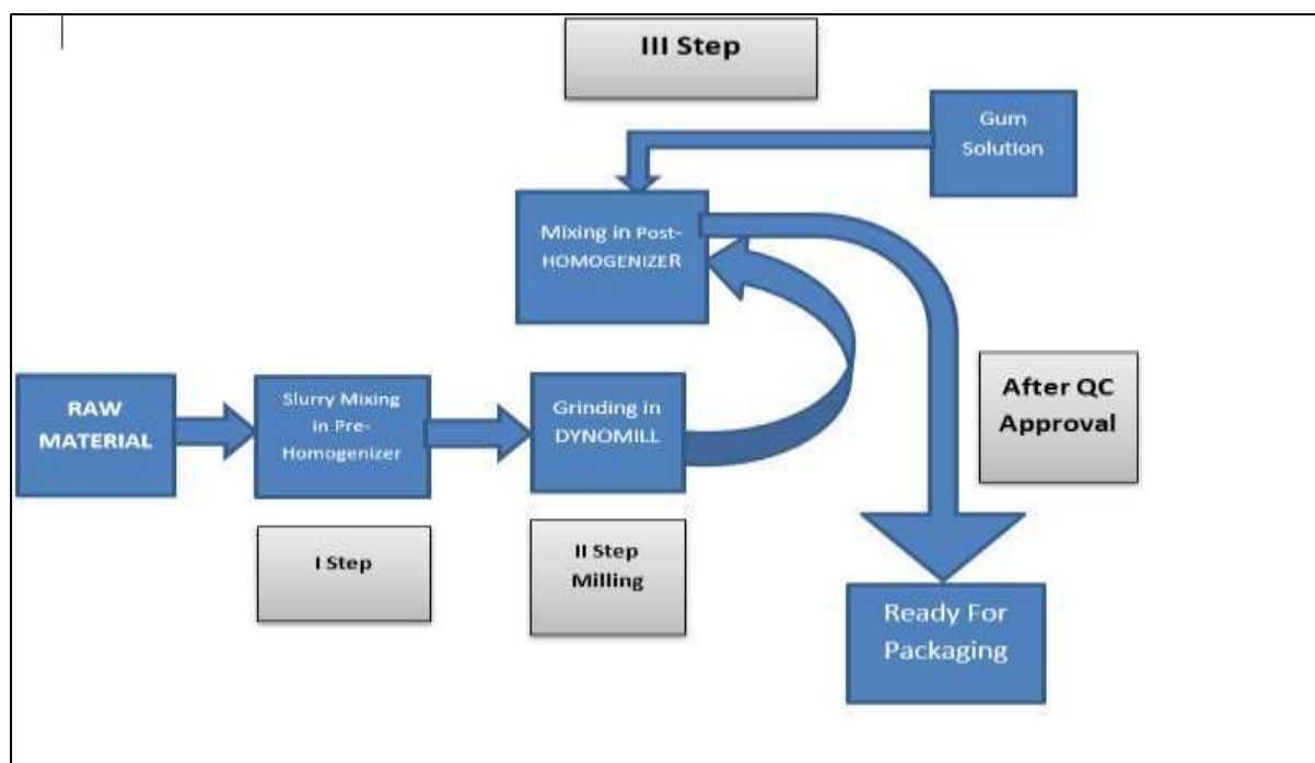
Manufacturing Process Flow Chart for WDG Formulation:
