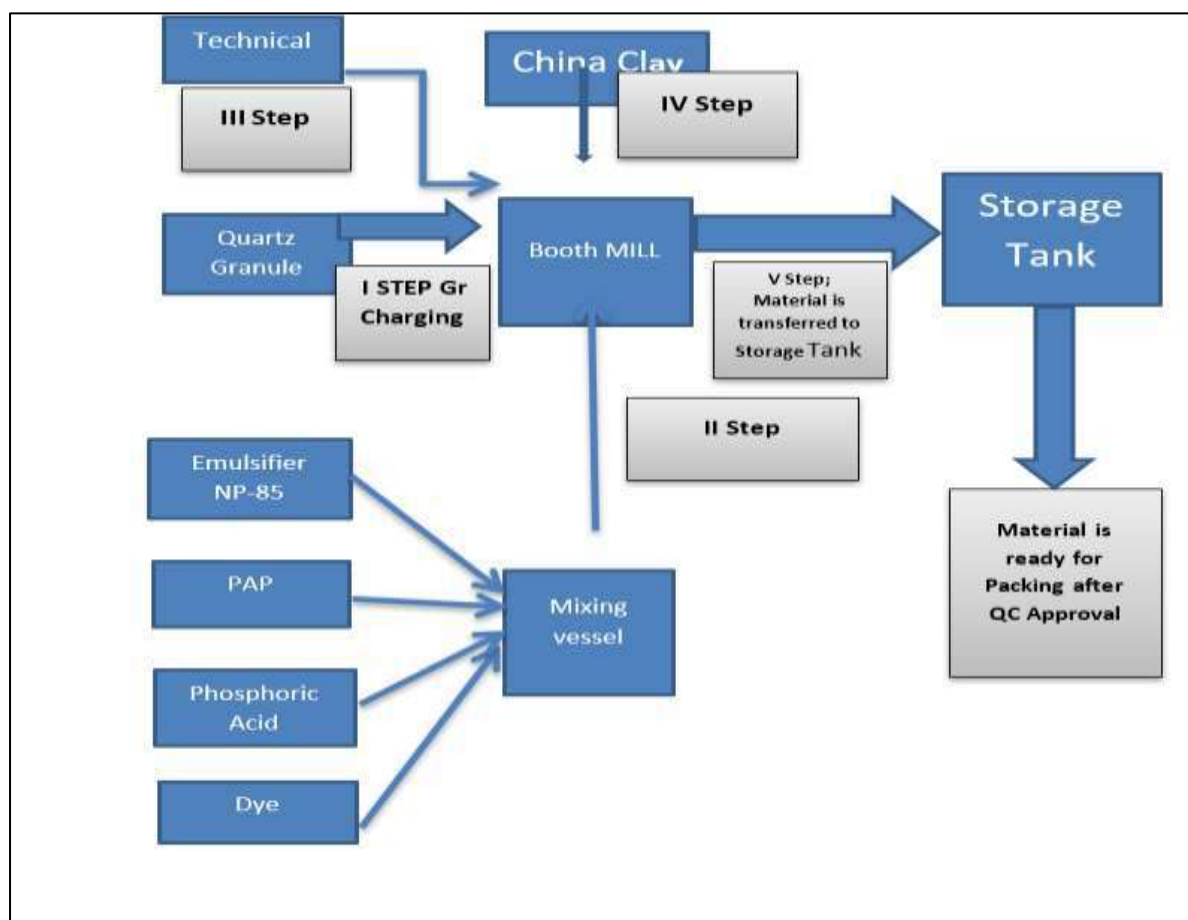
Manufacturing Process Flow Diagram for SC Formulation:
