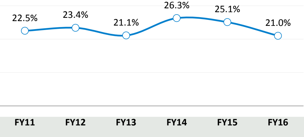
EBIT Margin (%)
