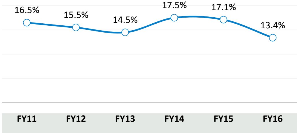
PAT Margin (%)
