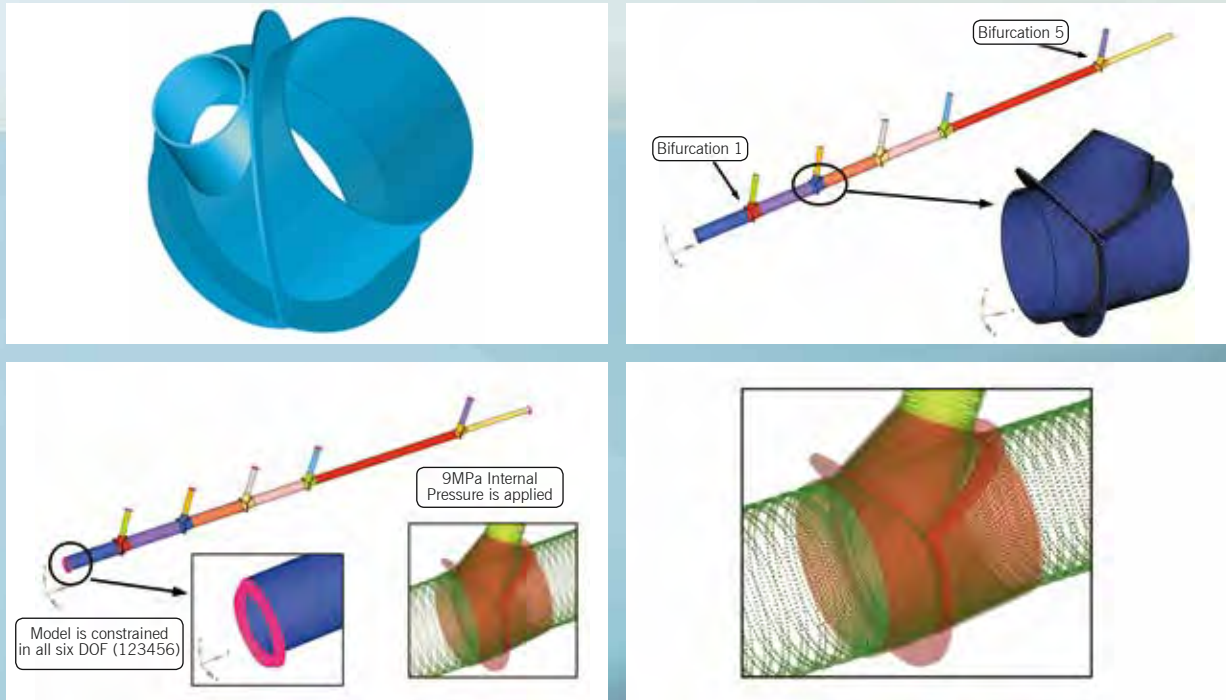
Finite Element Analysis (FEA) Models for Upper Tamakoshi HE Project, Nepal
