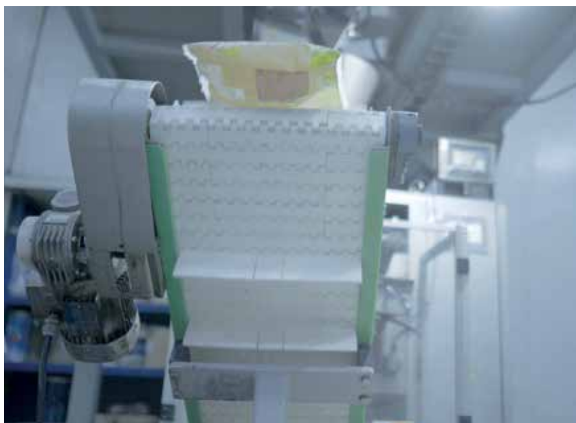
Amrit brand of Brown Sugar manufacturing at Nellikuppam
